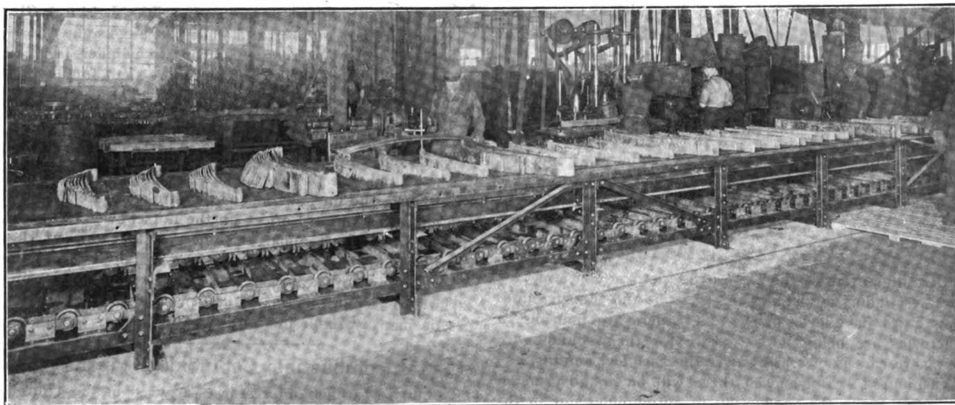
Movable assembly and inspection platform installed in the spring factory of the Detroit Steel Products Co., showing centrally the grinding of the spring ends, the third of 12 successive operations all performed on the platform
